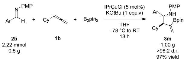
Scheme 3. Preparative scale copper-catalyzed borylative allylation of an imine. Ar = o -tolyl.
