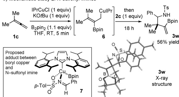
Scheme 4. a) The presence of an N-sulfonyl imine inhibits coupling with an N-phenyl imine. b) A preformed, functionalized allyl copper undergoes coupling with an N-sulfonyl imine. [21] Ts = 4-toluenesulfonyl.
