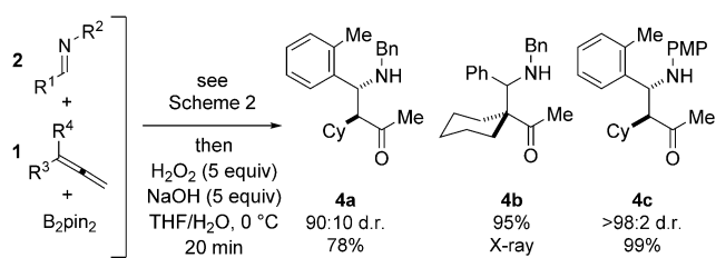
Figure 1. Copper-catalyzed three-component assembly of Mannich bases.
