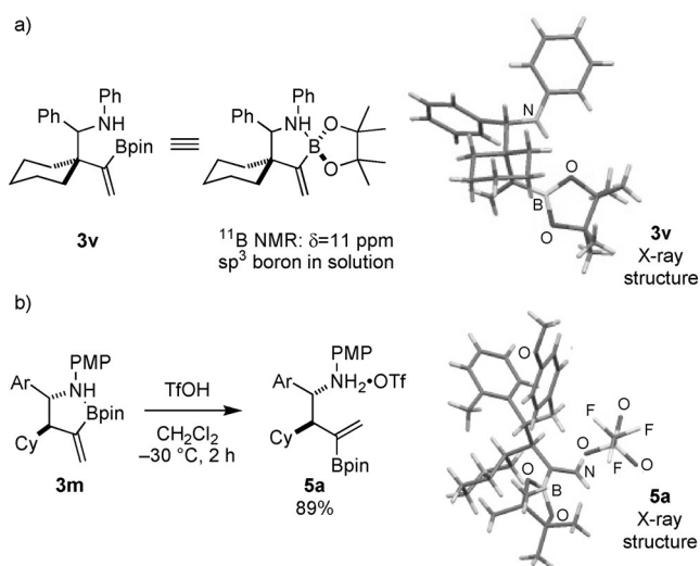
Figure 2. a) ^{11}\text{B} NMR data and X-ray crystallographic [21] analysis of 3v . b) Formation of a salt of 3m by disrupting the \text{N}_n \rightarrow \text{B}_p interaction. Ar = o -tolyl, Tf = trifluoromethanesulfonyl.
